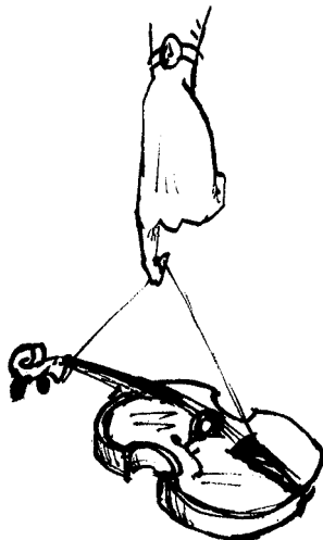
Pizzicato (Hilbert)
